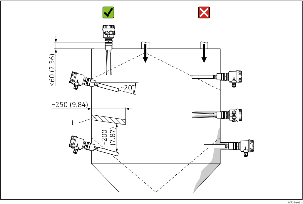
Unit of measurement mm (in) 1 Protective cover (provided by the customer)
